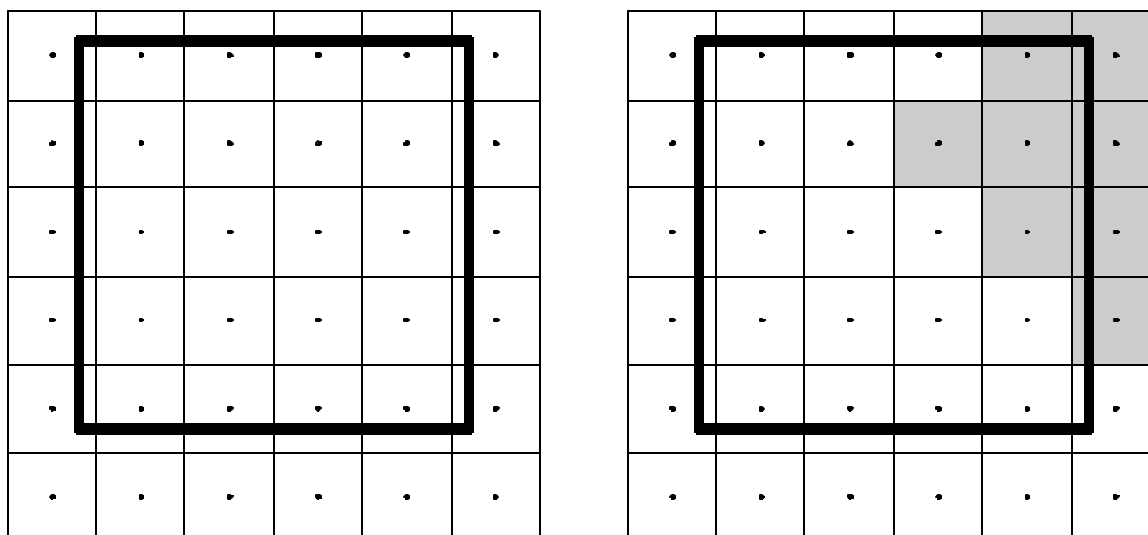
Figure 2. Data were resampled by locating which cells in the finer resolution grid (in this case, the NOHRSC at 1km) contained centerpoints within the bounds of the coarser grid (the NESDIS at just under 5km). If all of the NOHRSC cells had the same value (as in the figure on the left) the resampled grid was given that value. If all the NOHRSC cells falling within the bounds of a NESDIS cell were not homogenous (as in the figure on the right), the resampled grid was given the no-data value.
