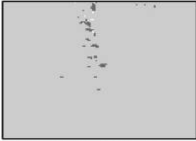
a) NOHRSC/MODIS northwest comparison for 3/23/2001 where forest density is between 75% and 100%.
