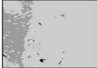
h) NOHRSC/MODIS northwest comparison for 3/26/2001 where forest density is between 0% and 25%.
