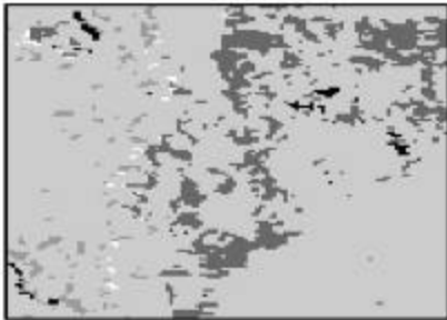
c) NOHRSC/MODIS northwest comparison for 3/23/2001 where forest density is between 25% and 50%..
