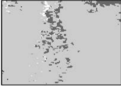
b) NOHRSC/MODIS northwest comparison for 3/23/2001 where forest density is between 50% and 75%.
