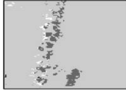
f) NOHRSC/MODIS northwest comparison for 3/26/2001 where forest density is between 50% and 75%.
