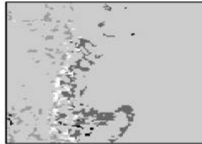
g) NOHRSC/MODIS northwest comparison for 3/26/2001 where forest density is between 25% and 50%.
