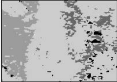
d) NOHRSC/MODIS northwest comparison for 3/23/2001 where forest density is between 0% and 25%.
